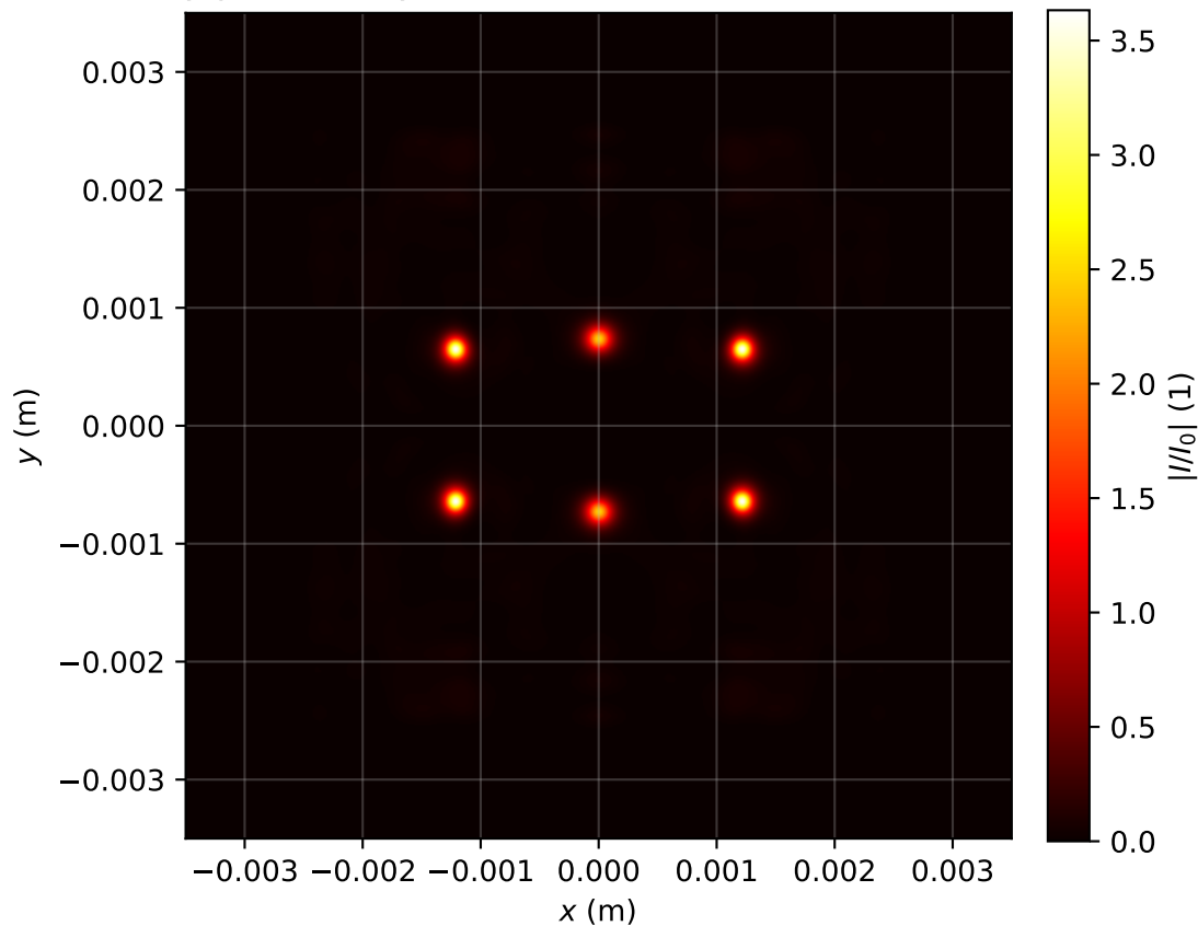
Intensity profile I(x, y, z = 2.707)/I_0 , P_{in}=12.0\text{Pcr} , artificial time
