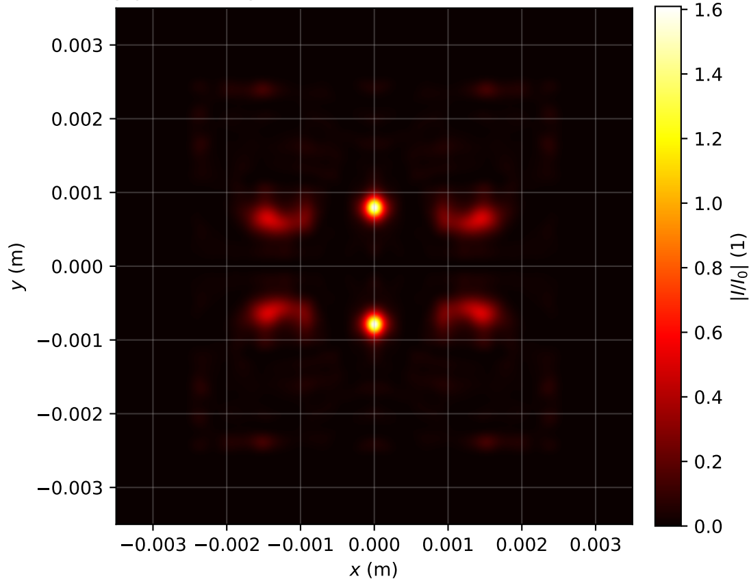
Intensity profile I(x, y, z = 3.184)/I_0 , P_{in}=12.0\text{Pcr} , artificial time
