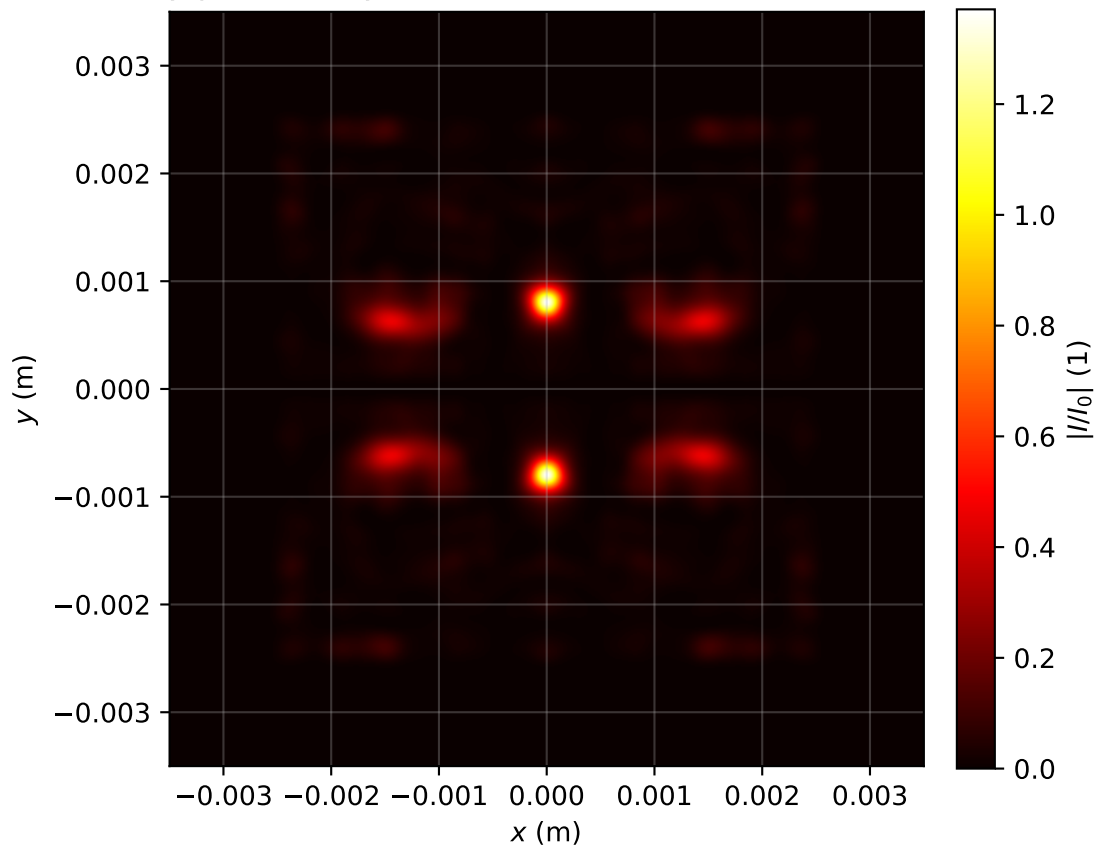
Intensity profile I(x, y, z = 3.264)/I_0 , P_{in}=12.0\text{Pcr} , artificial time
