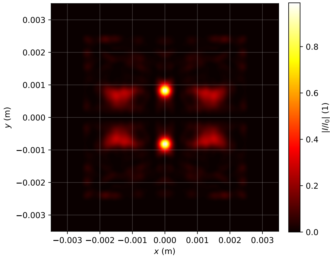
Intensity profile I(x, y, z = 3.423)/I_0 , P_{in}=12.0\text{Pcr} , artificial time
