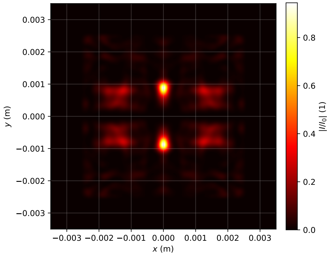
Intensity profile I(x, y, z = 3.582)/I_0 , P_{in}=12.0P_{cr} , artificial time
