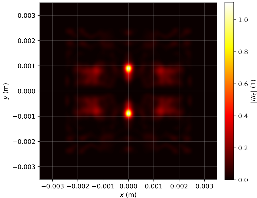
Intensity profile I(x, y, z = 3.662)/I_0 , P_{in}=12.0\text{Pcr} , artificial time
