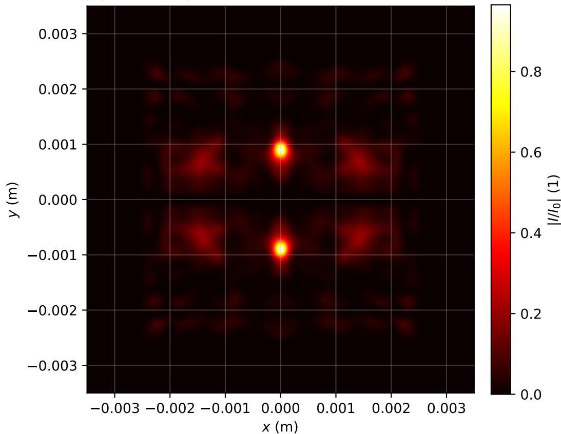
Intensity profile I(x, y, z = 3.821)/I_0 , P_{in}=12.0P_{cr} , artificial time
