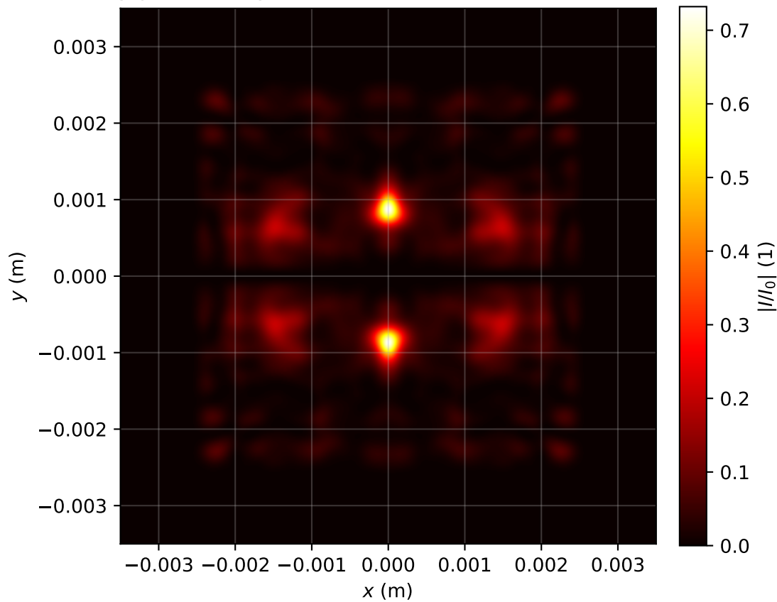
Intensity profile I(x, y, z = 3.901)/I_0 , P_{in}=12.0\text{Pcr} , artificial time
