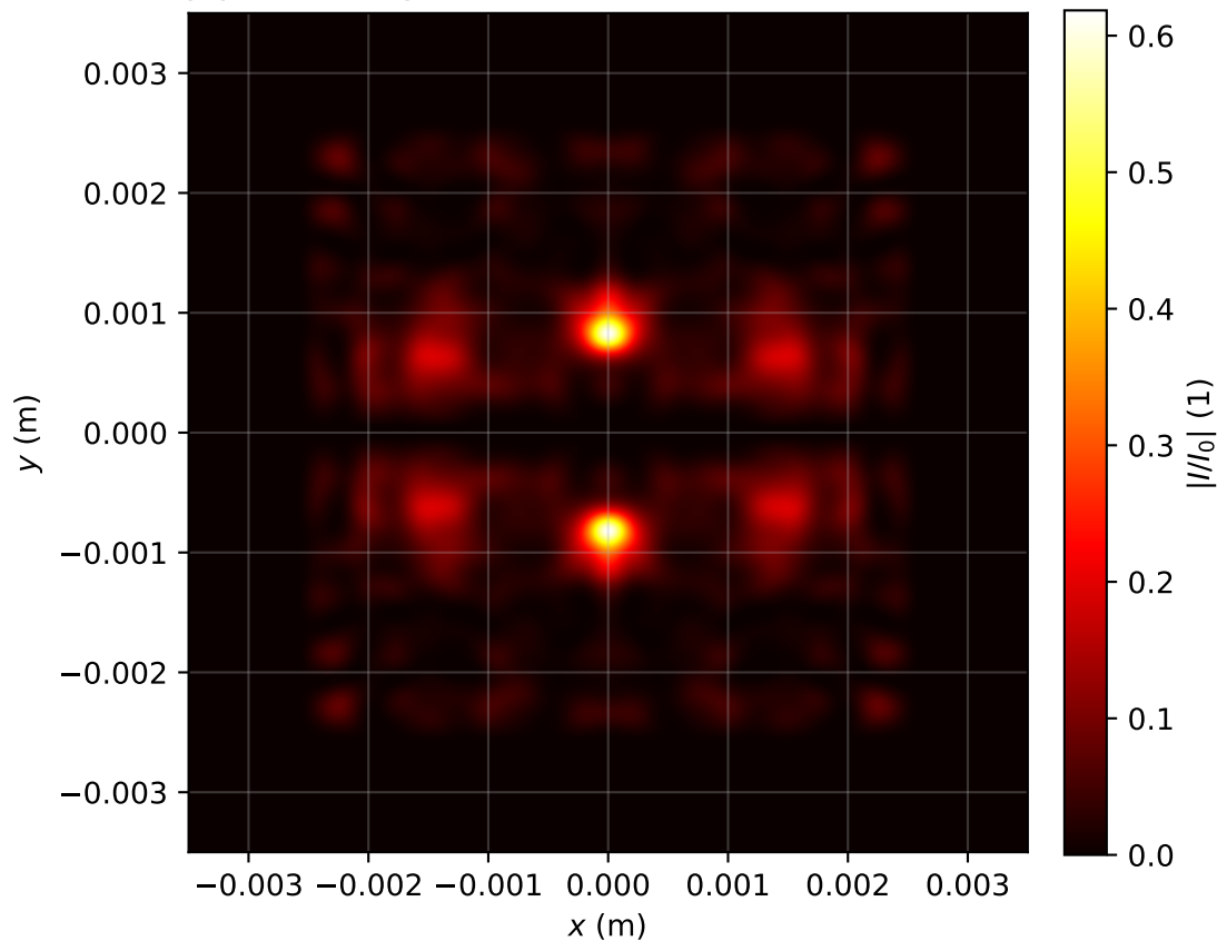
Intensity profile I(x, y, z = 3.981)/I_0 , P_{in}=12.0\text{Pcr} , artificial time
