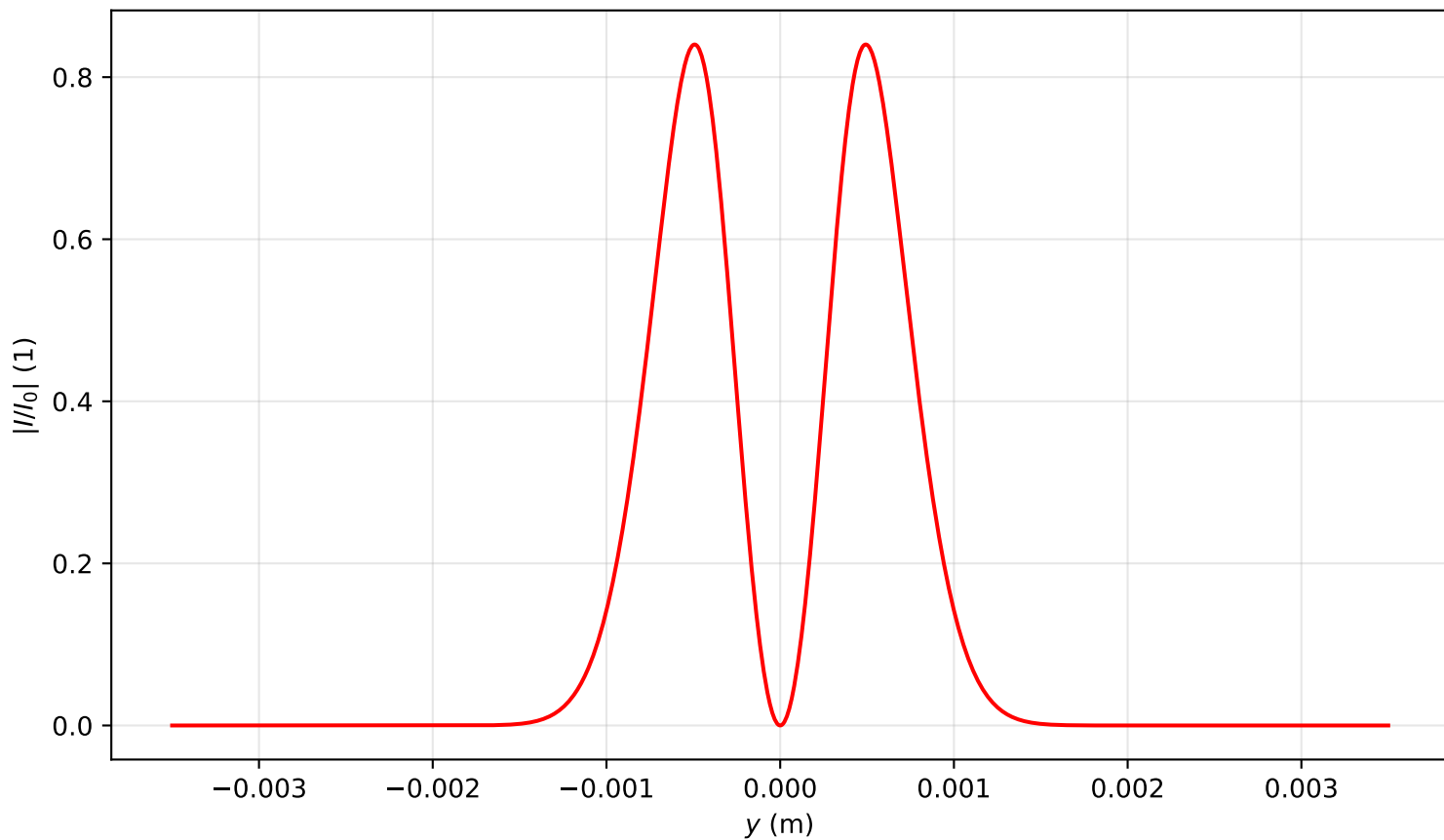
Intensity profile I(x=0, y, z=0.080)/I_0 , P_{in}=12.0P_{cr} , artificial time
