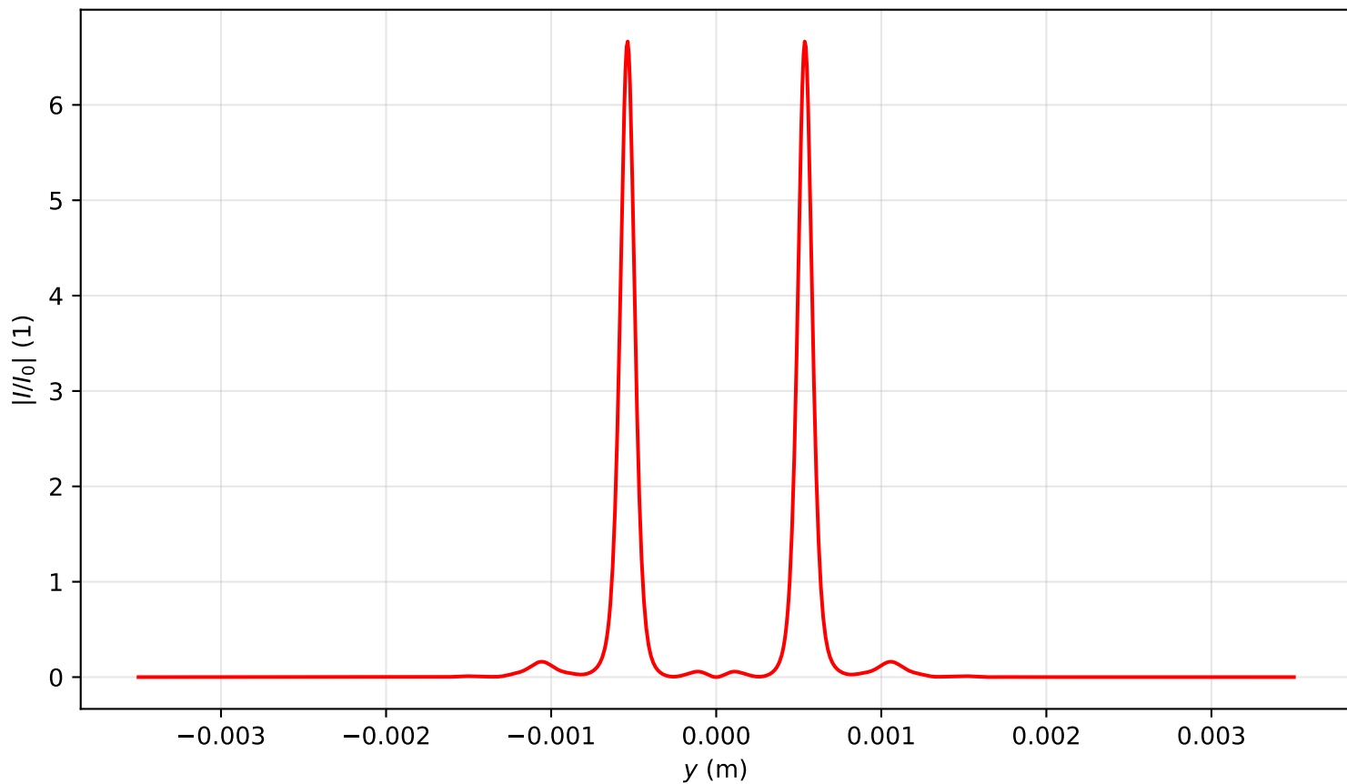
Intensity profile I(x = 0, y, z = 0.716)/I_0 , P_{in}=12.0\text{Pcr} , artificial time
