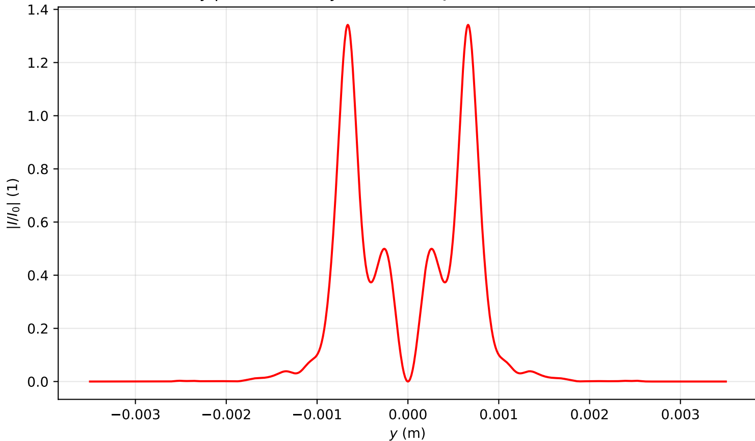
Intensity profile I(x=0, y, z=1.194)/I_0 , P_{in}=12.0P_{cr} , artificial time
