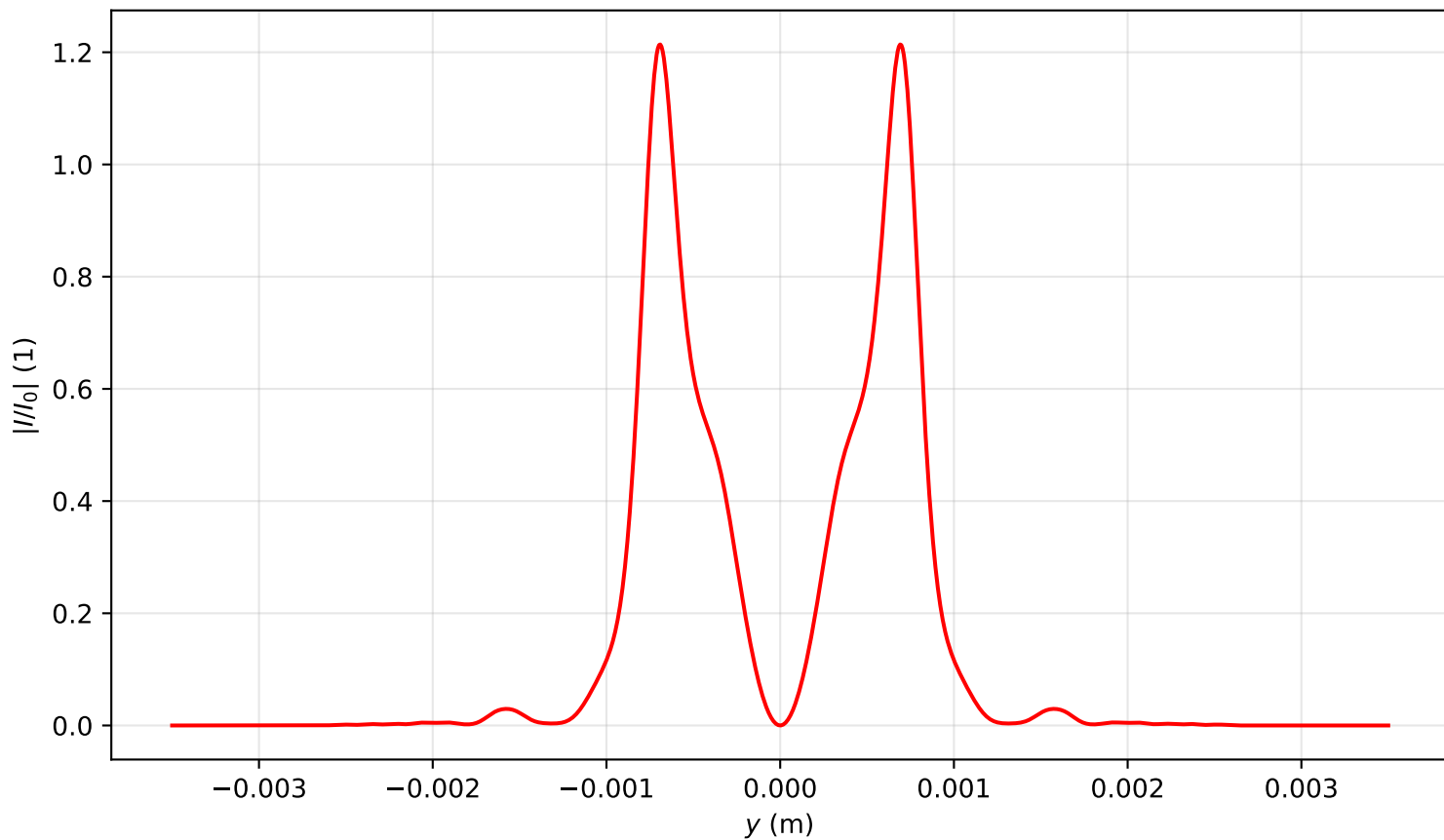
Intensity profile I(x=0, y, z=1.353)/I_0 , P_{in}=12.0P_{cr} , artificial time
