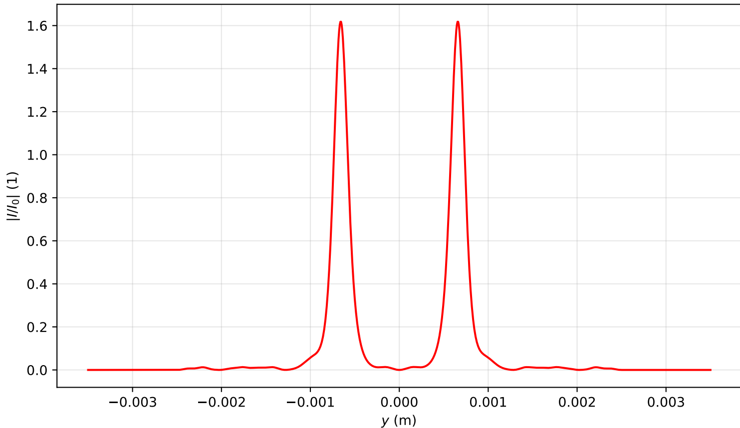
Intensity profile I(x=0, y, z=1.751)/I_0 , P_{in}=12.0P_{cr} , artificial time
