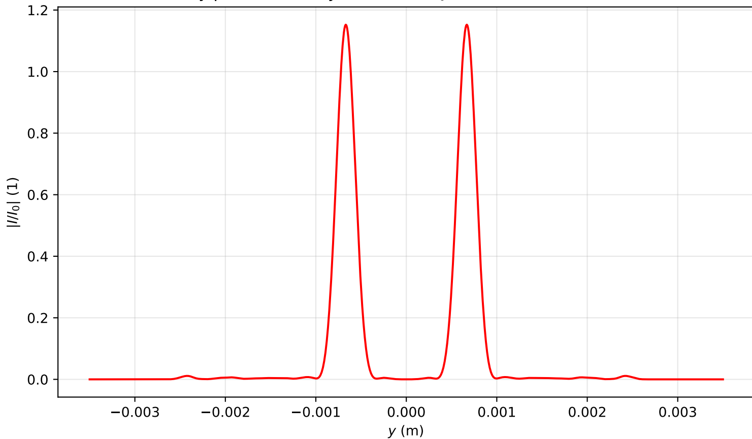
Intensity profile I(x=0, y, z=1.831)/I_0 , P_{in}=12.0P_{cr} , artificial time
