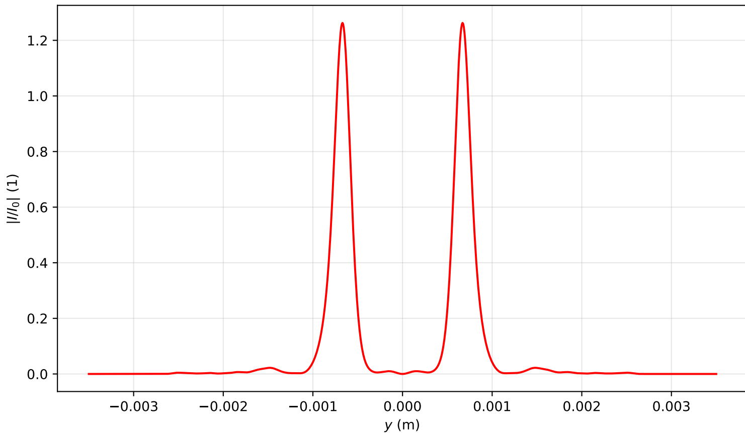
Intensity profile I(x=0, y, z=1.911)/I_0 , P_{in}=12.0P_{cr} , artificial time
