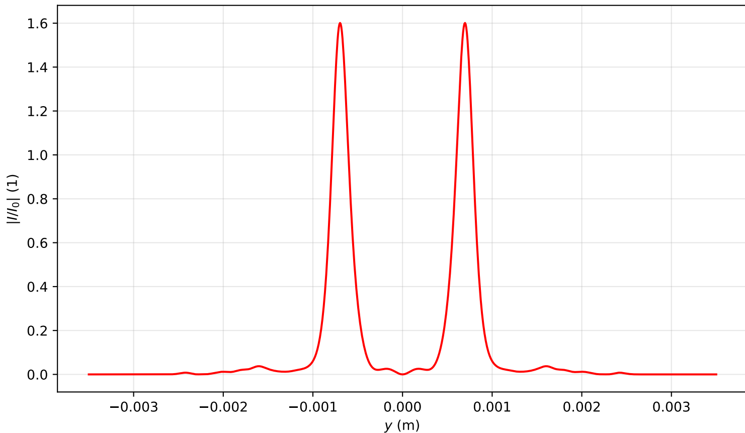
Intensity profile I(x=0, y, z=1.990)/I_0 , P_{in}=12.0P_{cr} , artificial time
