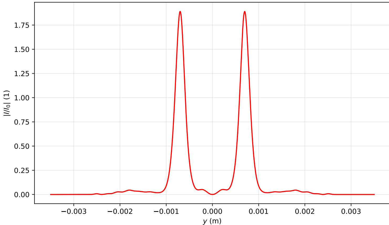
Intensity profile I(x=0, y, z=2.070)/I_0 , P_{in}=12.0P_{cr} , artificial time
