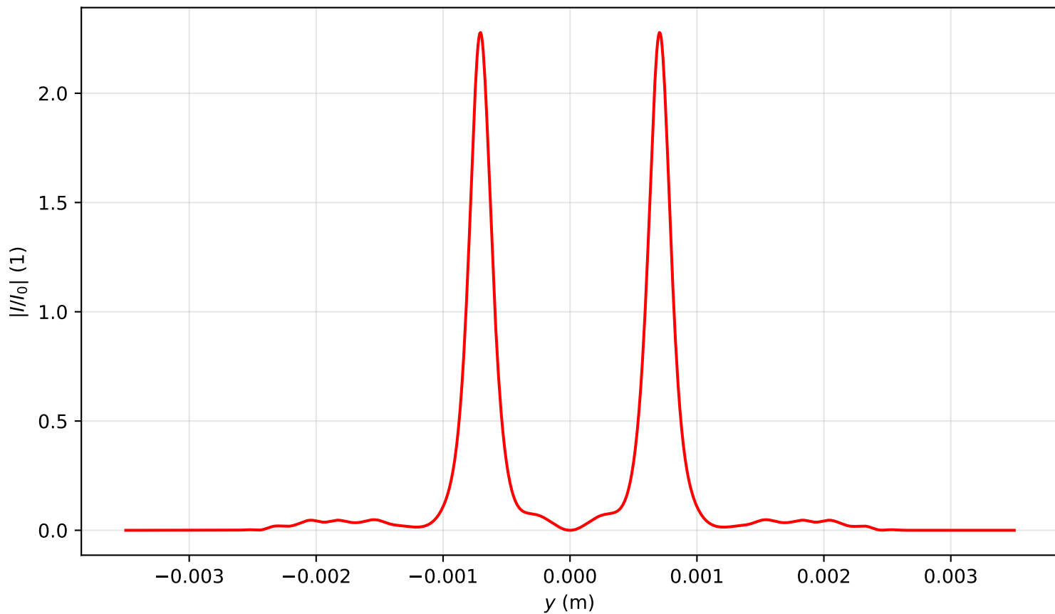
Intensity profile I(x=0, y, z=2.149)/I_0 , P_{in}=12.0P_{cr} , artificial time
