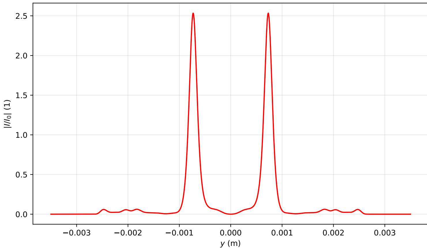
Intensity profile I(x=0, y, z=2.388)/I_0 , P_{in}=12.0P_{cr} , artificial time
