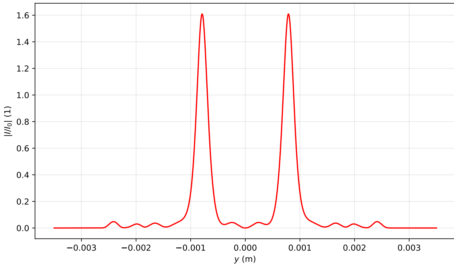
Intensity profile I(x=0, y, z=3.184)/I_0 , P_{in}=12.0P_{cr} , artificial time
