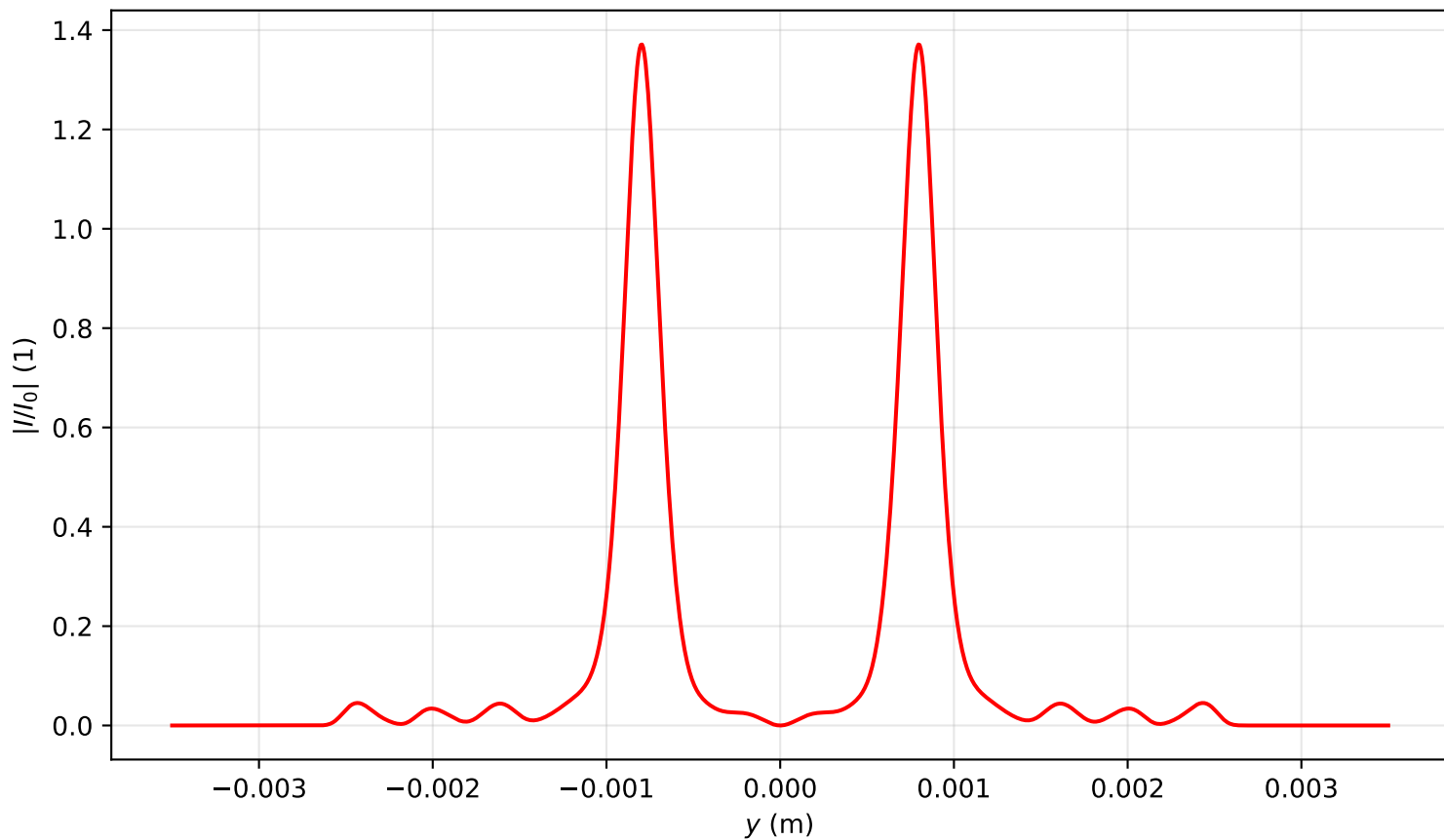
Intensity profile I(x=0, y, z=3.264)/I_0 , \text{Pin}=12.0\text{Pcr} , artificial time
