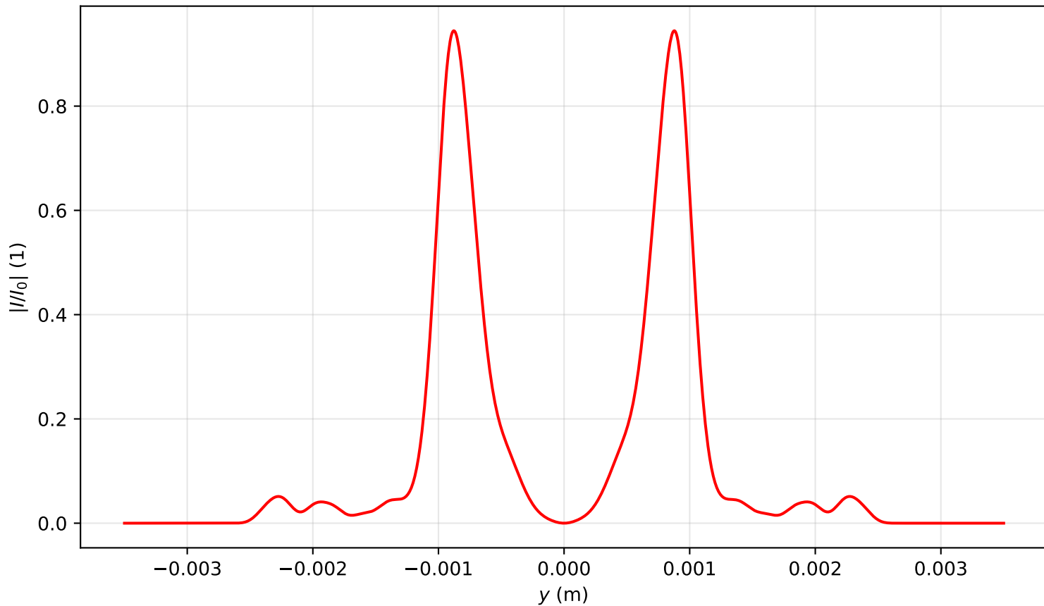
Intensity profile I(x=0, y, z=3.582)/I_0 , P_{in}=12.0P_{cr} , artificial time
