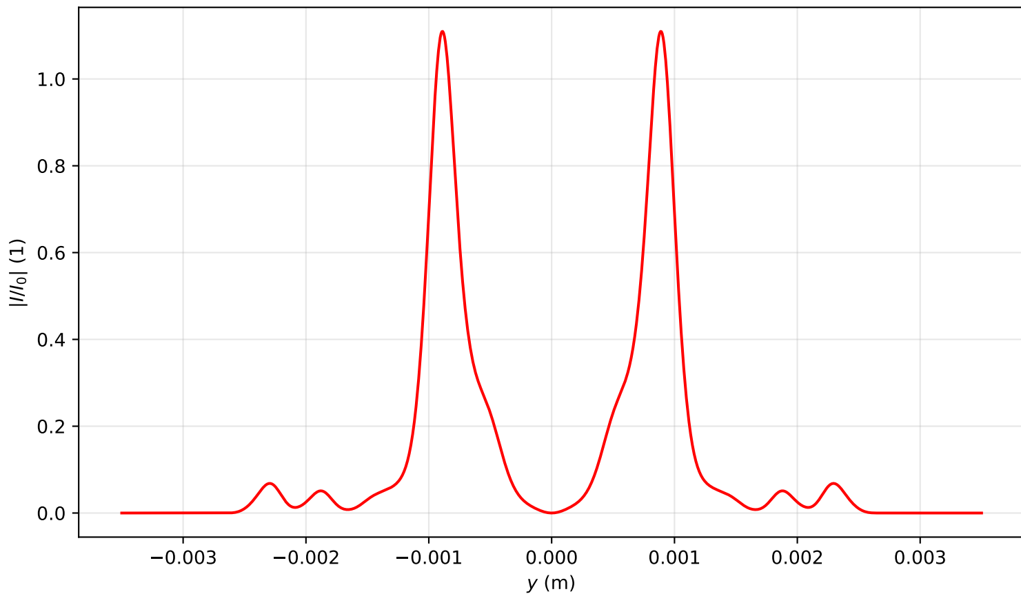
Intensity profile I(x=0, y, z=3.662)/I_0 , P_{in}=12.0P_{cr} , artificial time
