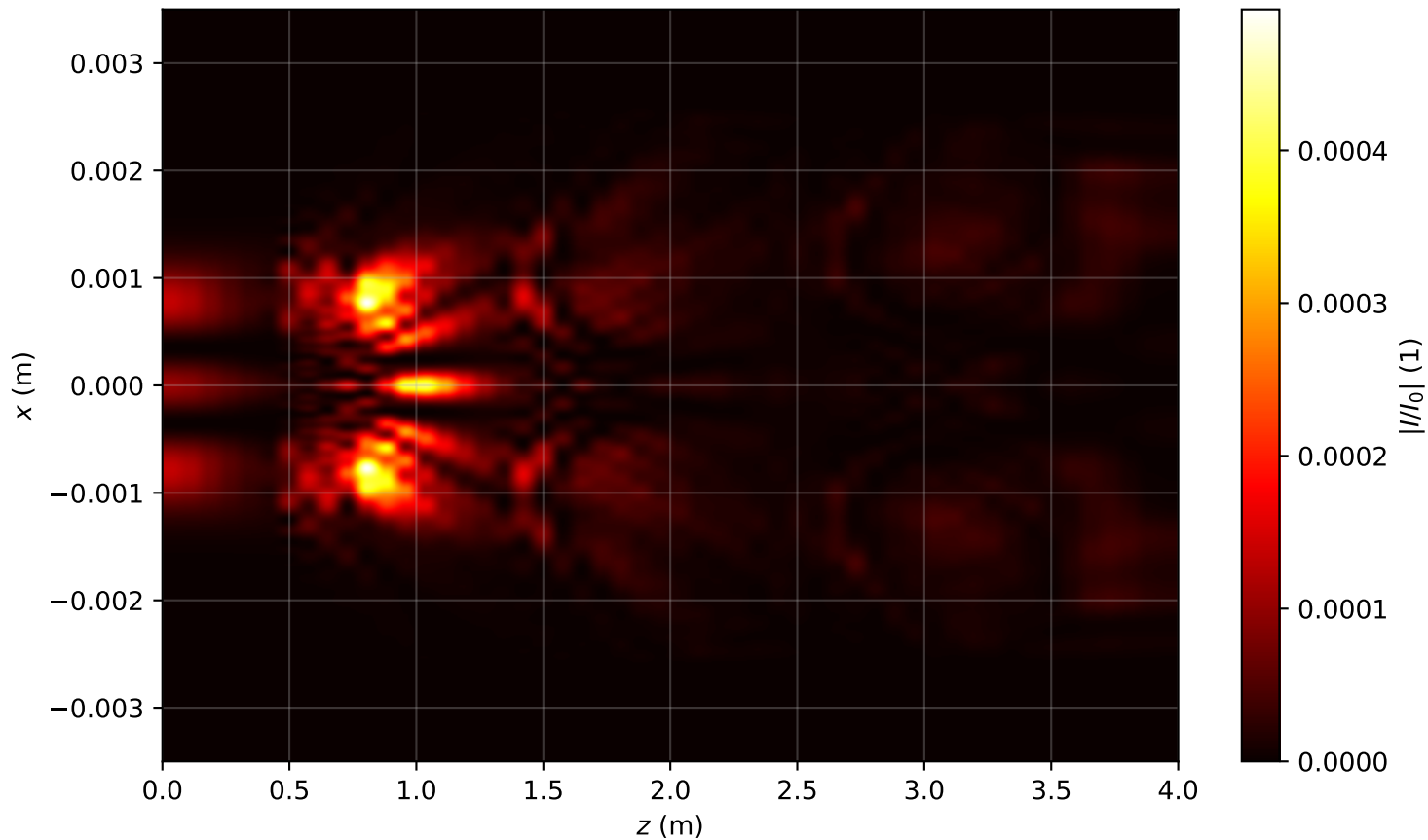
Intensity profile I(x, y = 0, z)/I_0 , P_{in}=12.0P_{cr} , artificial time
