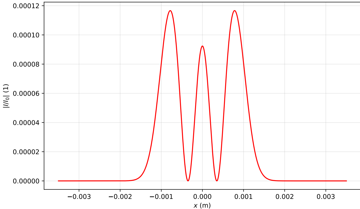
Intensity profile I(x, y = 0, z = 0.080)/I_0 , P_{in}=13.0P_{cr} , artificial time
