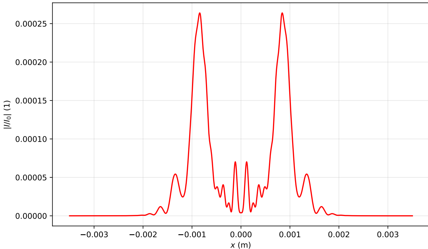
Intensity profile I(x, y = 0, z = 0.557)/I_0 , P_{in}=13.0P_{cr} , artificial time
