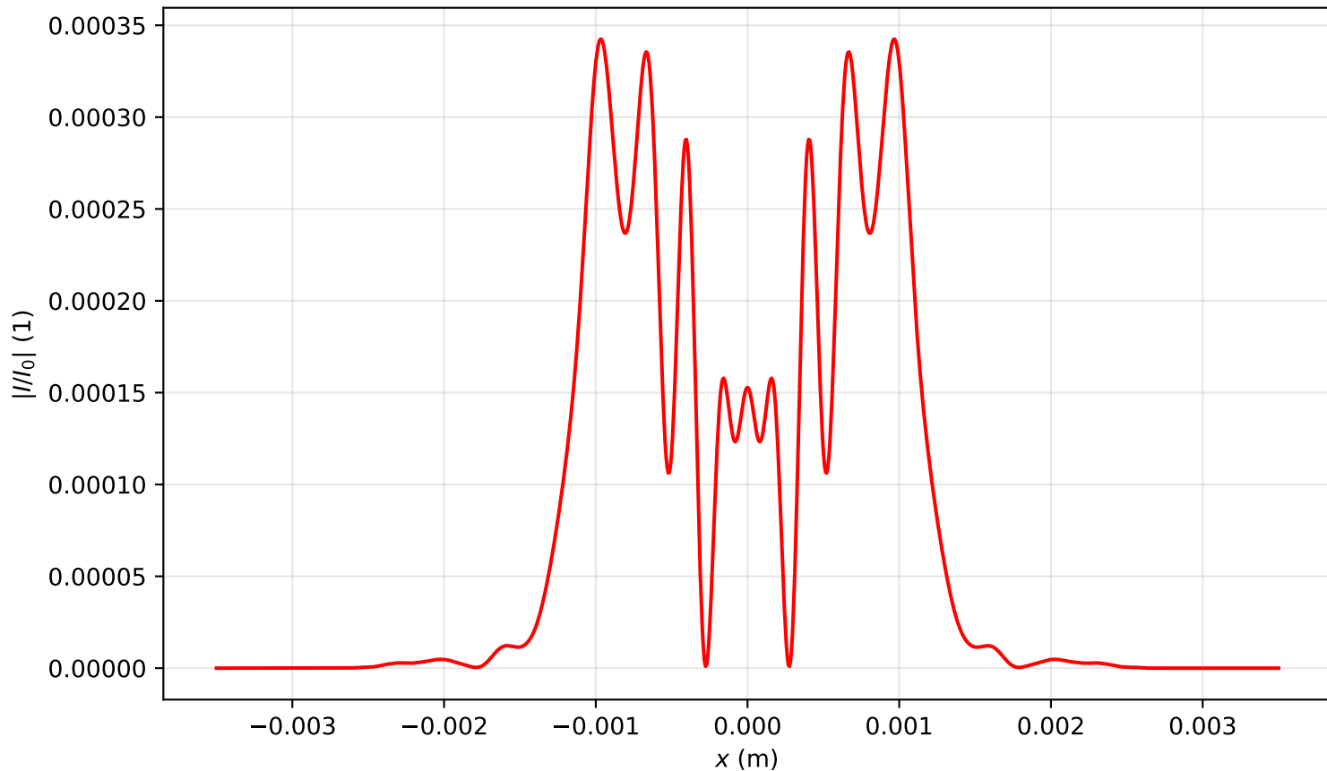
Intensity profile I(x, y = 0, z = 0.876)/I_0 , P_{in}=13.0P_{cr} , artificial time
