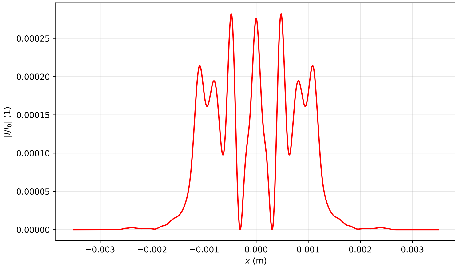
Intensity profile I(x, y = 0, z = 0.955)/I_0 , P_{in}=13.0P_{cr} , artificial time
