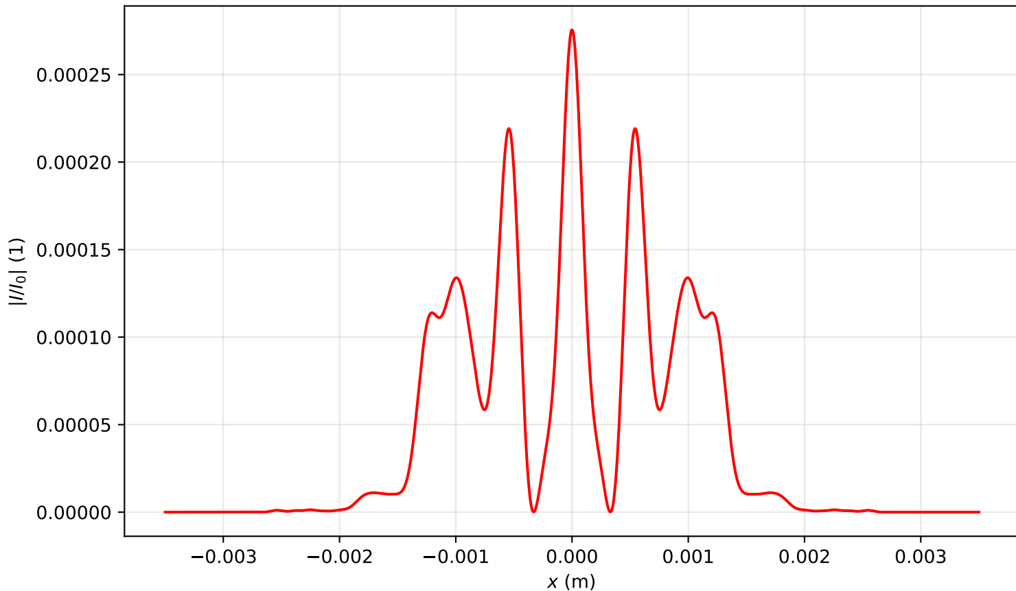
Intensity profile I(x, y = 0, z = 1.035)/I_0 , P_{in}=13.0P_{cr} , artificial time
