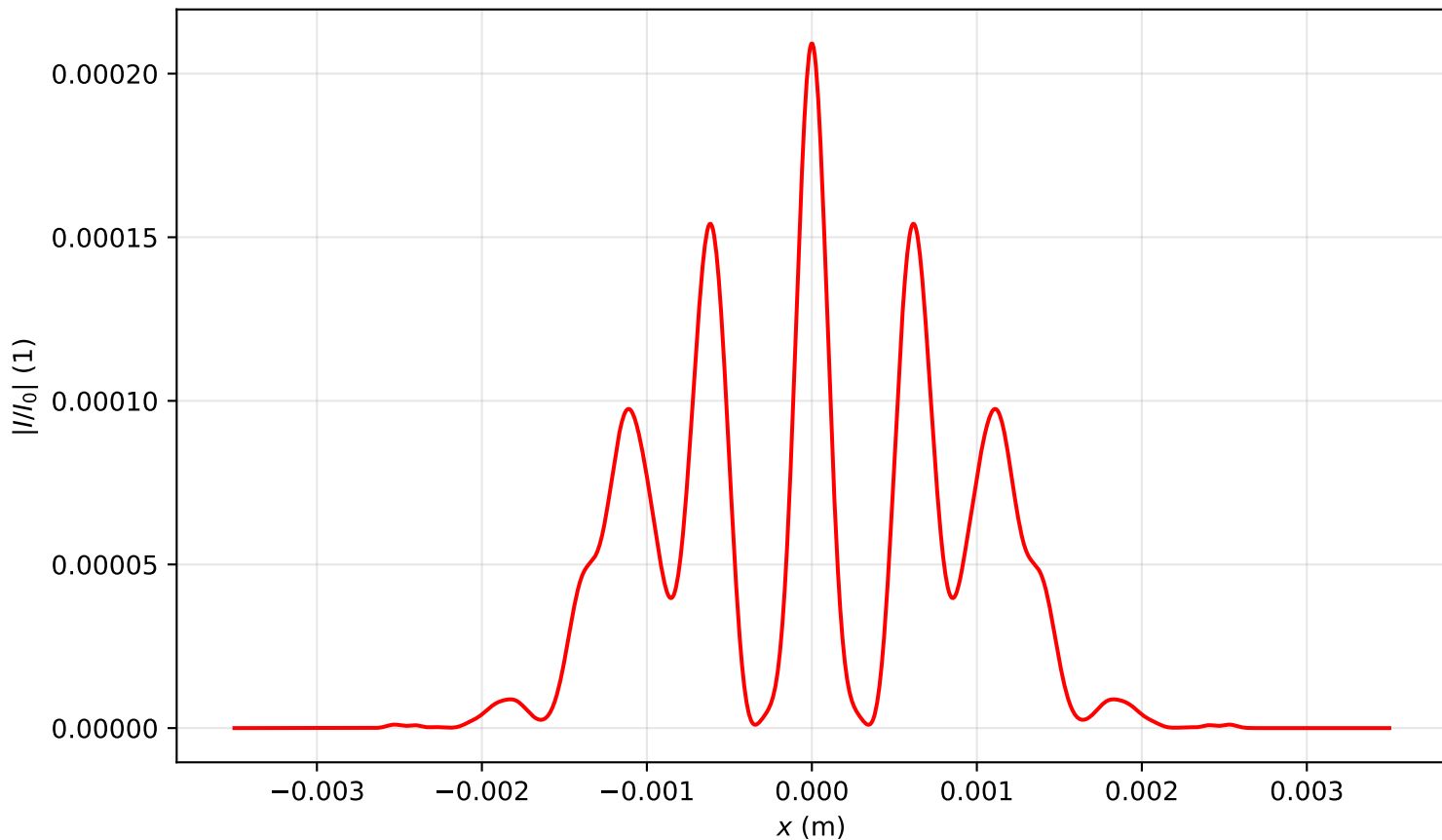
Intensity profile I(x, y = 0, z = 1.115)/I_0 , P_{in}=13.0P_{cr} , artificial time
