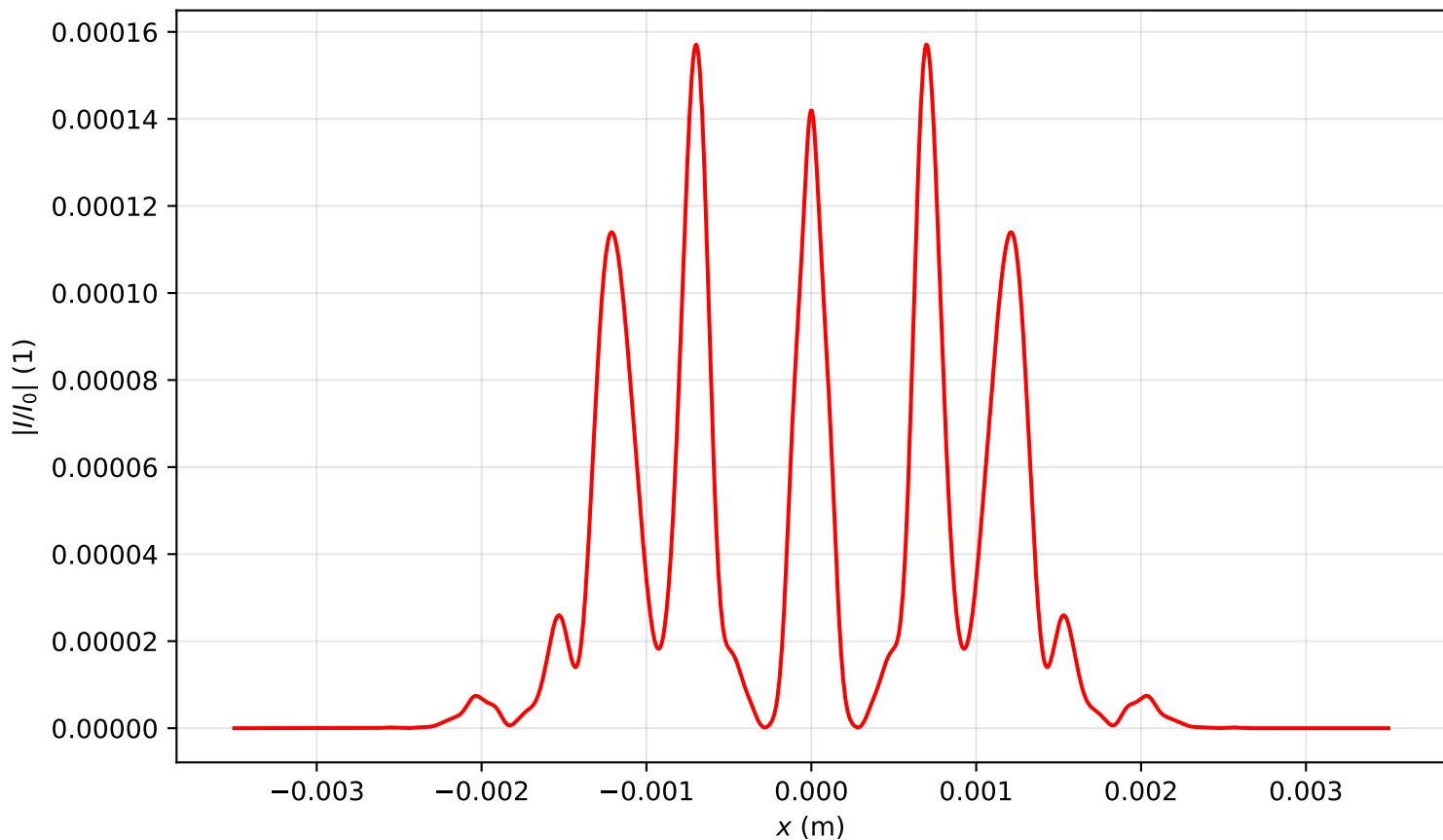
Intensity profile I(x, y = 0, z = 1.194)/I_0 , P_{in}=13.0P_{cr} , artificial time
