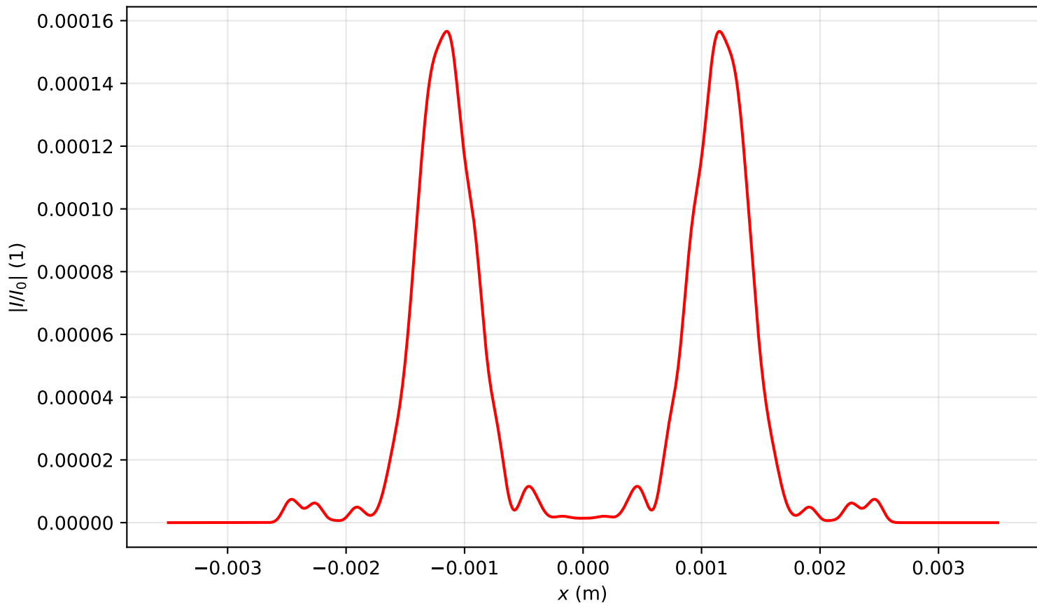
Intensity profile I(x, y = 0, z = 2.309)/I_0 , P_{in}=13.0P_{cr} , artificial time
