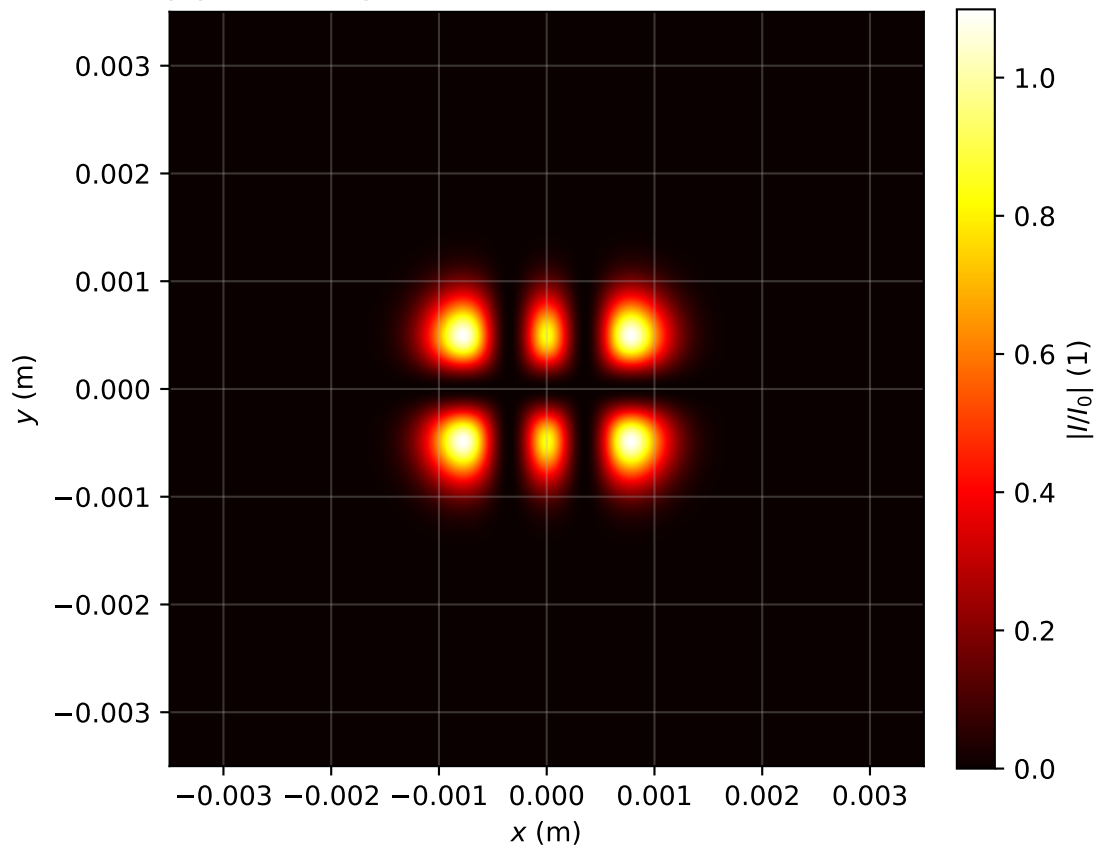
Intensity profile I(x, y, z = 0.080)/I_0 , P_{in}=13.0\text{Pcr} , artificial time
