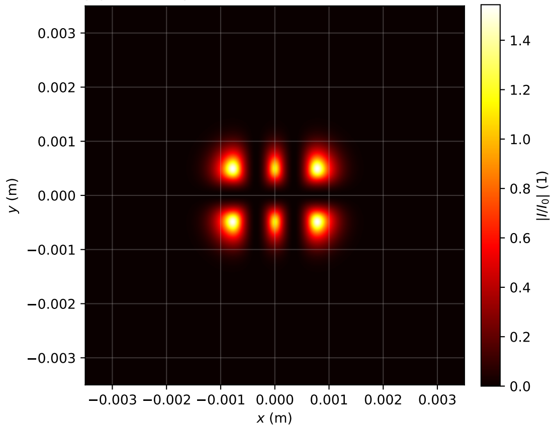
Intensity profile I(x, y, z = 0.159)/I_0 , P_{in}=13.0\text{Pcr} , artificial time
