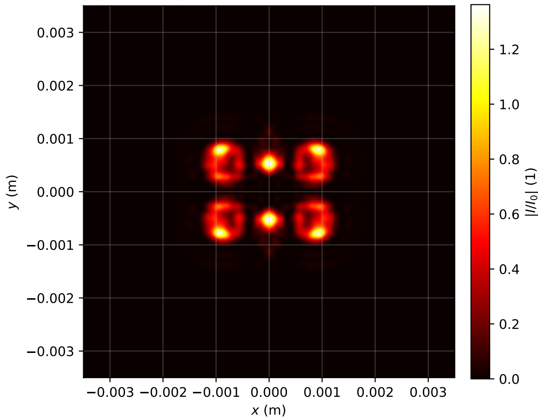
Intensity profile I(x, y, z = 0.716)/I_0 , P_{in}=13.0P_{cr} , artificial time
