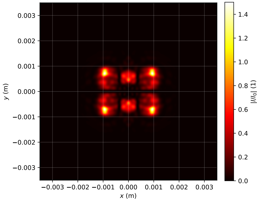
Intensity profile I(x, y, z = 0.796)/I_0 , P_{in}=13.0\text{Pcr} , artificial time
