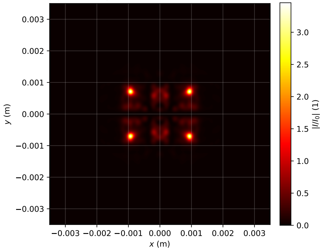
Intensity profile I(x, y, z = 0.955)/I_0 , P_{in}=13.0P_{cr} , artificial time
