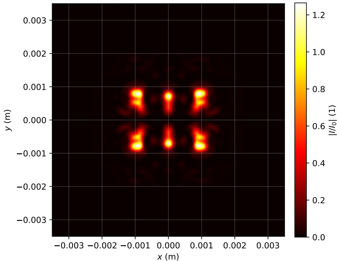
Intensity profile I(x, y, z = 1.274)/I_0 , P_{in}=13.0\text{Pcr} , artificial time
