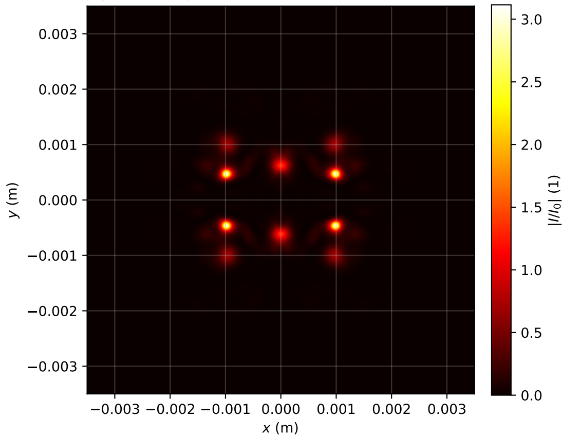
Intensity profile I(x, y, z = 1.513)/I_0 , P_{in}=13.0P_{cr} , artificial time
