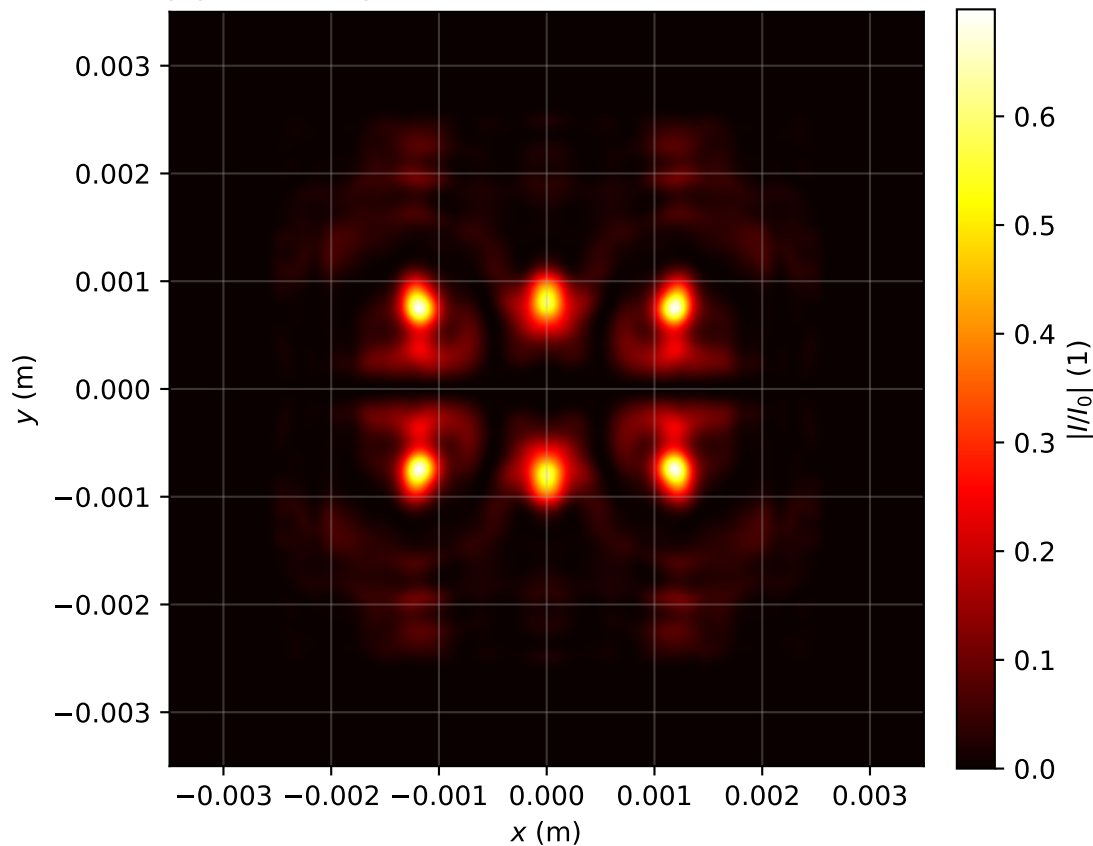
Intensity profile I(x, y, z = 2.548)/I_0 , P_{in}=13.0\text{Pcr} , artificial time
