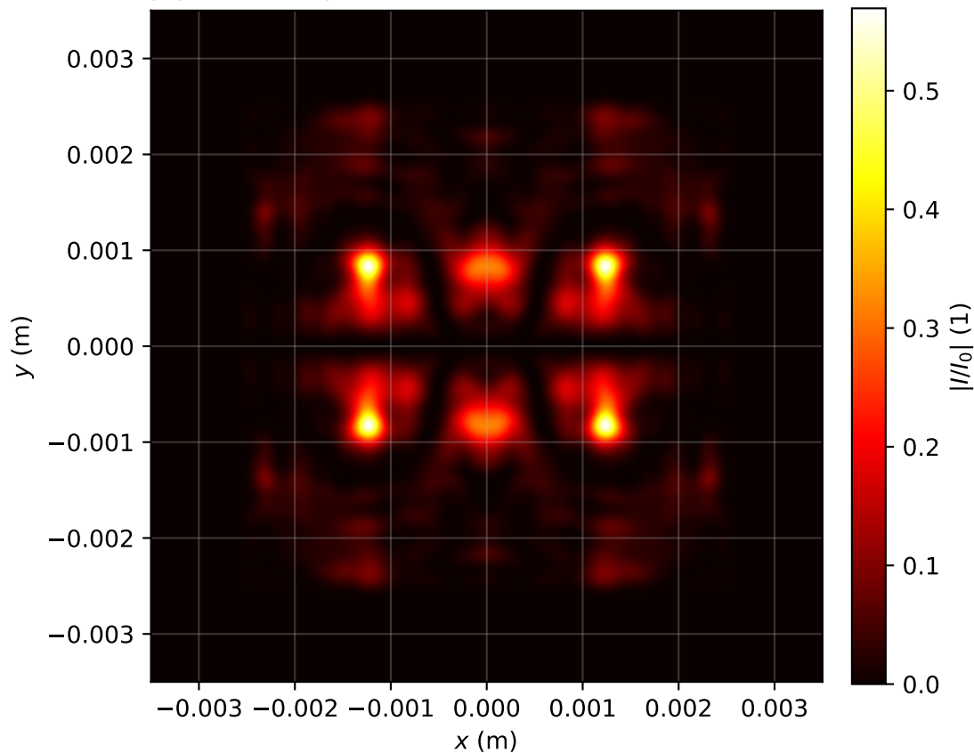
Intensity profile I(x, y, z = 2.707)/I_0 , P_{in}=13.0P_{cr} , artificial time
