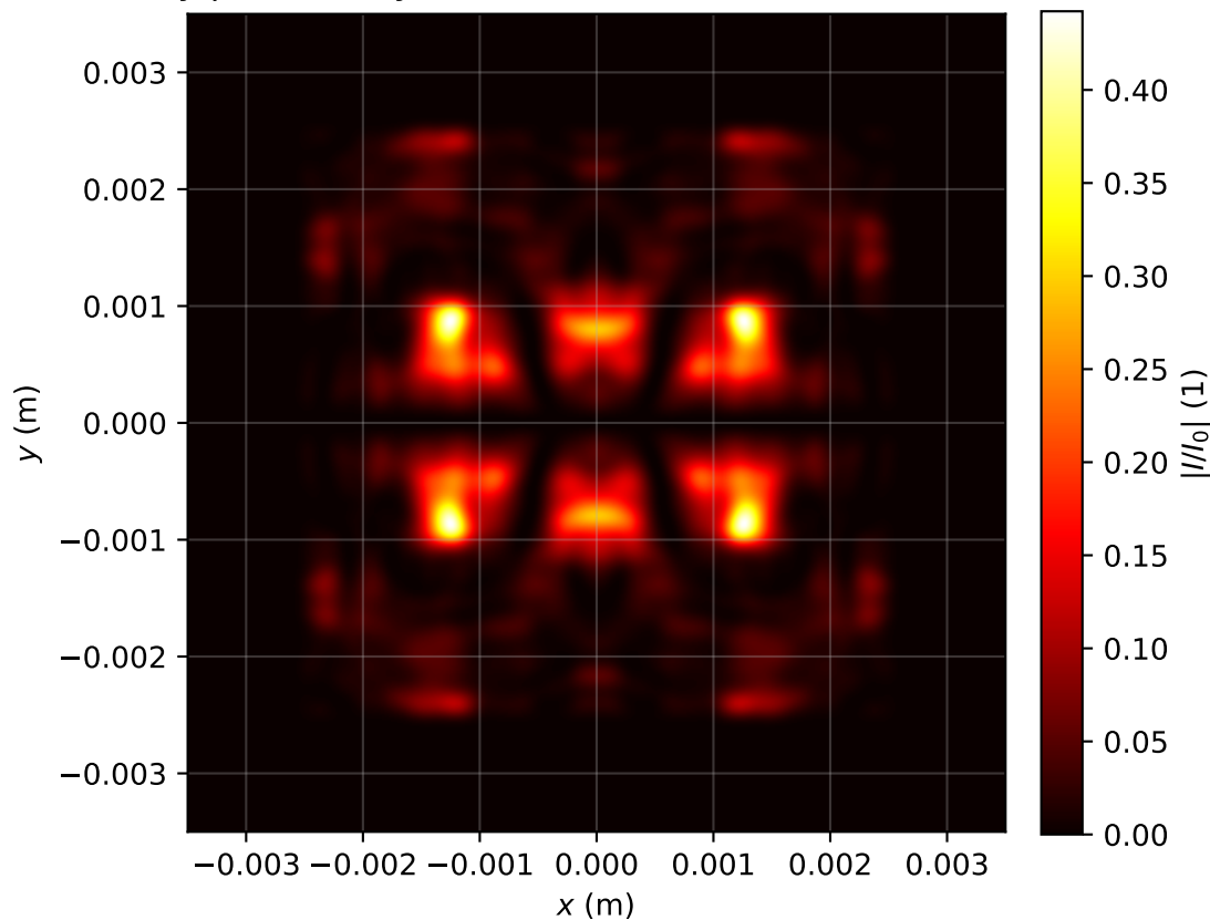
Intensity profile I(x, y, z = 2.786)/I_0 , P_{in}=13.0P_{cr} , artificial time
