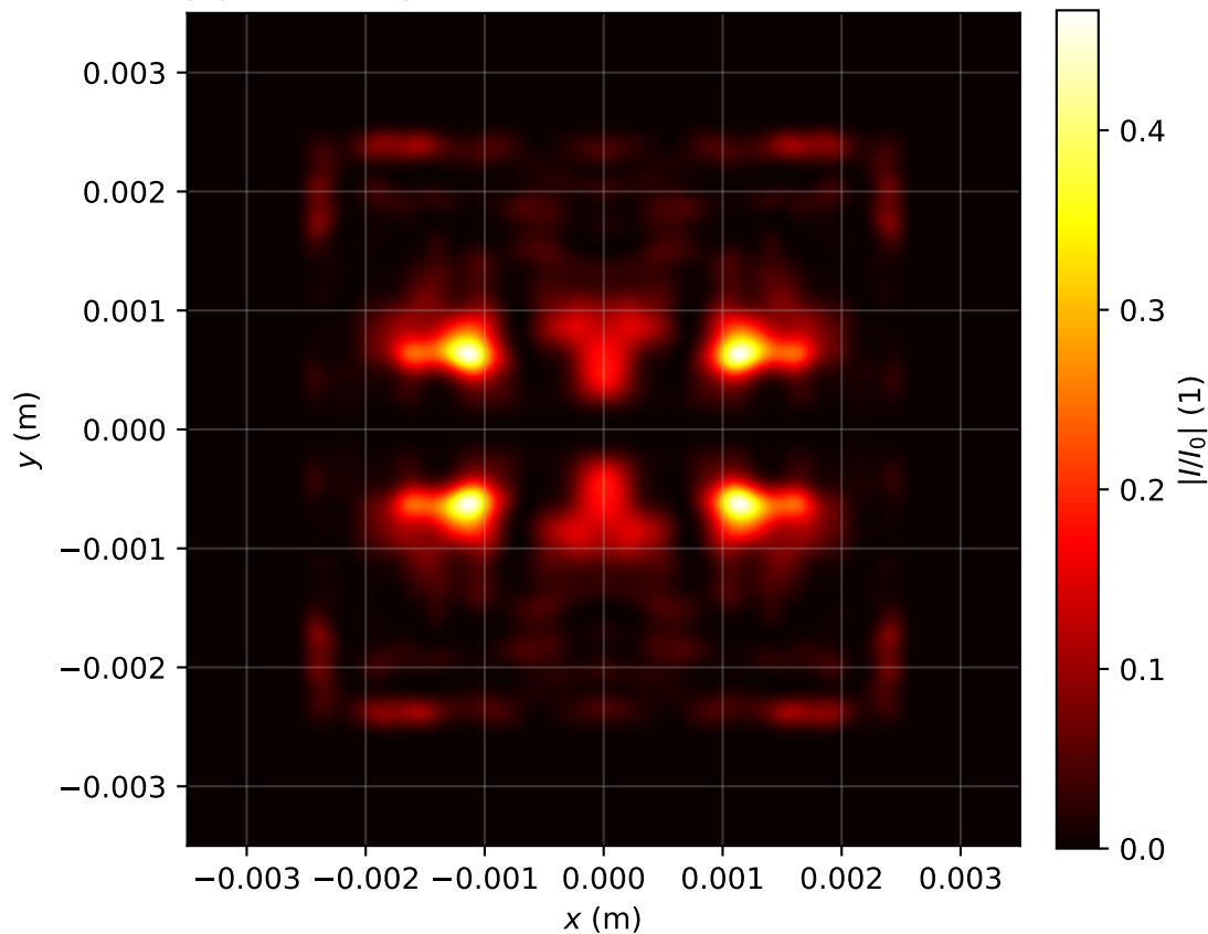
Intensity profile I(x, y, z = 3.264)/I_0 , P_{in}=13.0\text{Pcr} , artificial time
