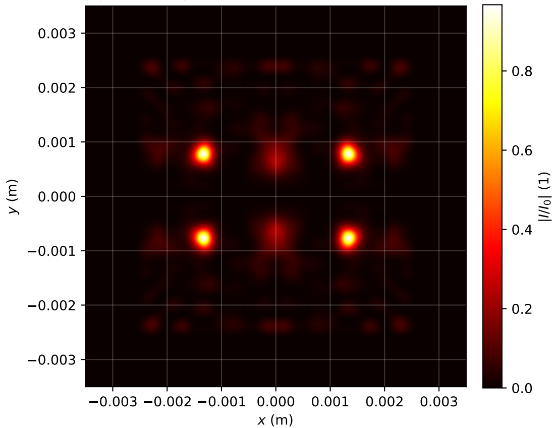
Intensity profile I(x, y, z = 3.901)/I_0 , P_{in}=13.0P_{cr} , artificial time
