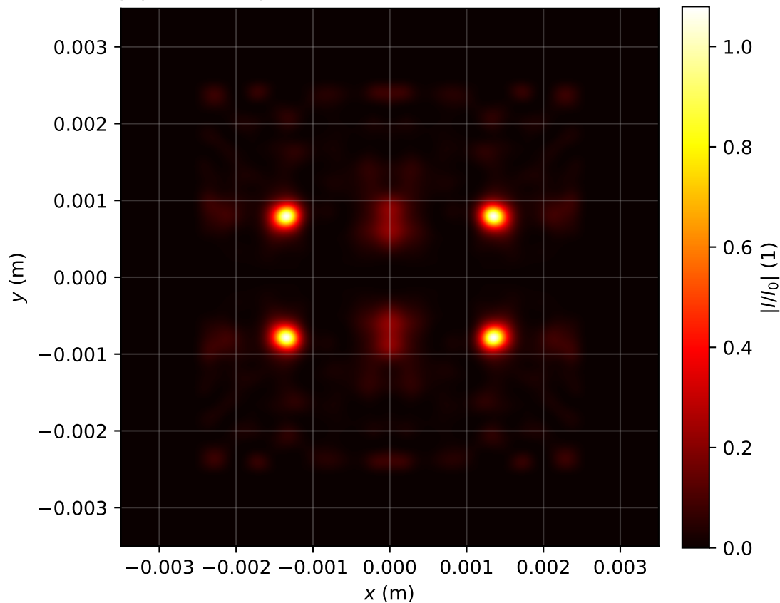
Intensity profile I(x, y, z = 3.981)/I_0 , P_{in}=13.0\text{Pcr} , artificial time
