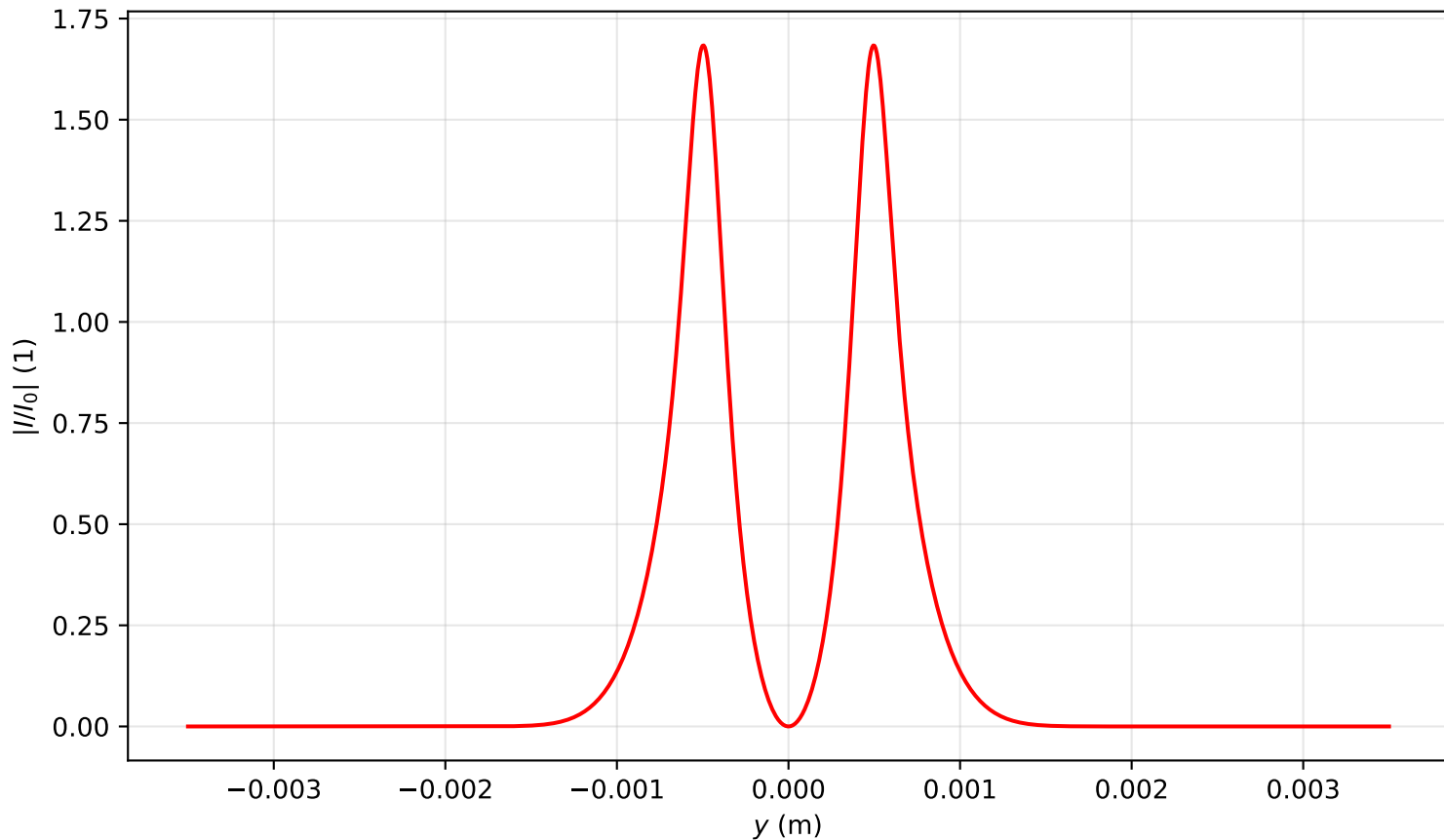
Intensity profile I(x = 0, y, z = 0.239)/I_0 , P_{in}=13.0P_{cr} , artificial time
