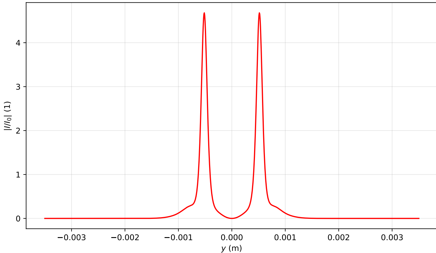
Intensity profile I(x=0, y, z=0.398)/I_0 , P_{in}=13.0P_{cr} , artificial time
