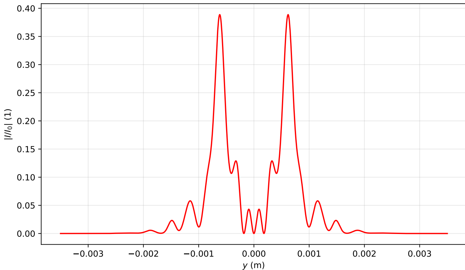
Intensity profile I(x = 0, y, z = 0.876)/I_0 , P_{in}=13.0P_{cr} , artificial time
