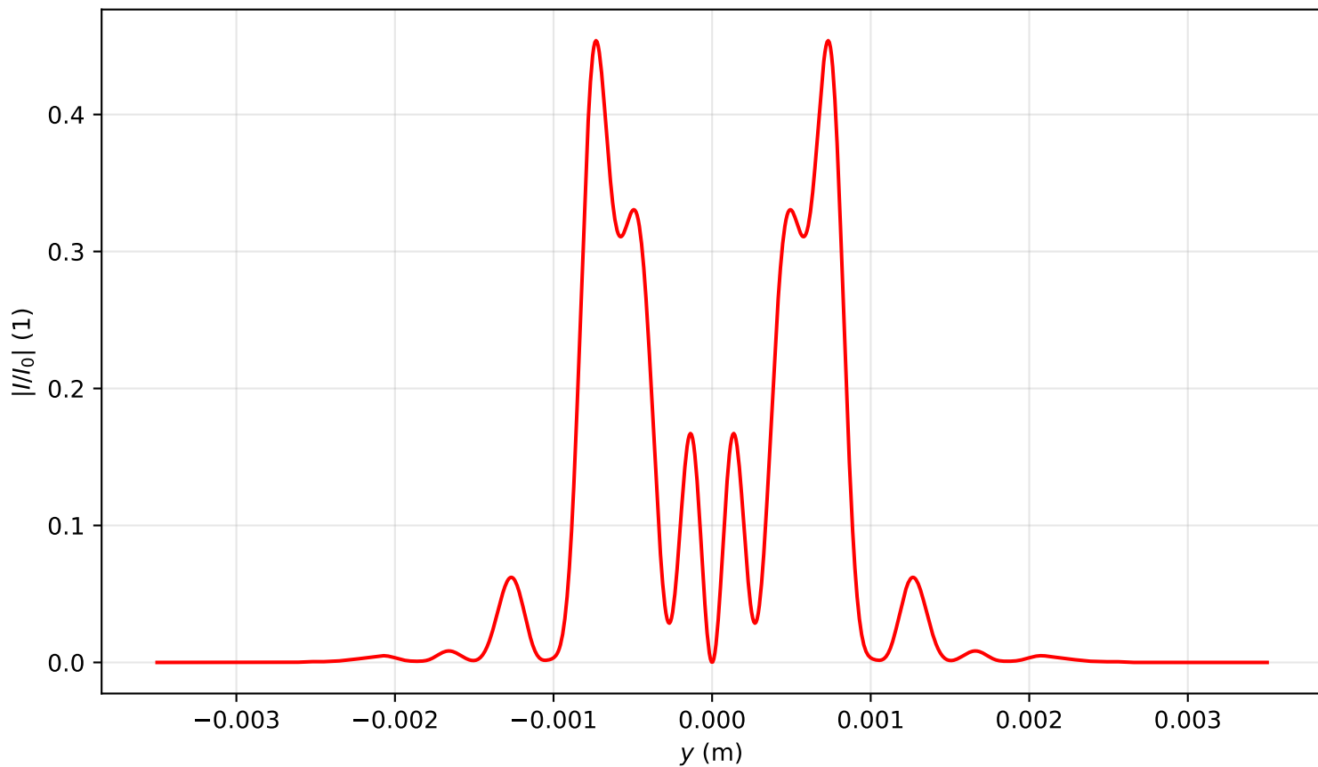
Intensity profile I(x=0, y, z=0.955)/I_0 , P_{in}=13.0\text{Pcr} , artificial time
